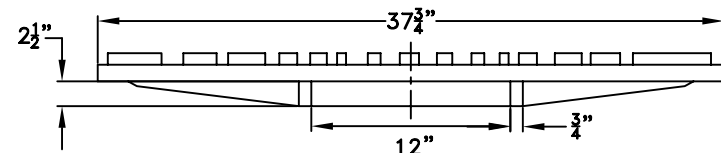
MANHOLE COVER
