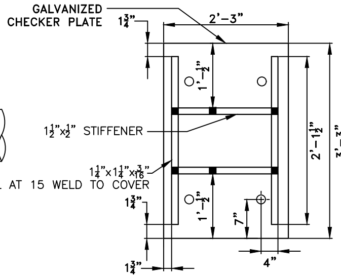
(UNDERSIDE) PLAN
