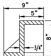
DETAIL 1
